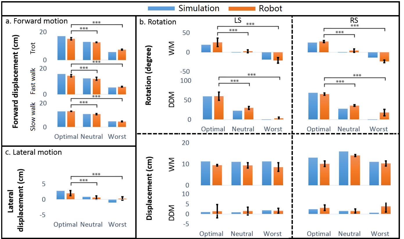
Fig. 6. Experiment results of RFT simulations (blue) and robot experiments (orange) of (a) forward, (b) rotational and (c) lateral gaits, showing close agreement between simulations and experiments. Each gait is tested for 3 experiment trials, each containing at least 3 gait periods. The “optimal”, “neutral” and “worst” respectively represent optimal back bending, no back bending and worst back bending. Means and standard deviations can be found in the supplement materials. We indicate statistically significant [52] improvement, when comparing the ‘optimal’-‘neutral’, as well as ‘optimal’-‘worst’ gaits (* : p < .05 , ** : p < .01 , *** p < .001 ). For LS (lateral sequence), RS (rotary sequence), DDM (differential drive machine) and WM (walking machine), we show both displacement and rotation values for completeness only: back bending is optimized wrt. rotation only, and displacement changes are not meaningful.
